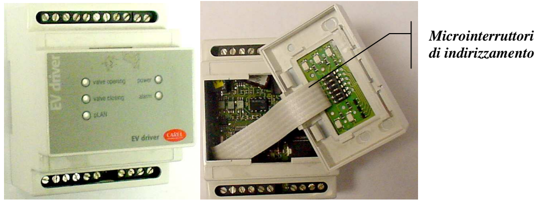
Fig. 7 – Driver EEXV
