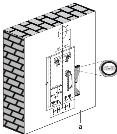
a Pared plana vertical
