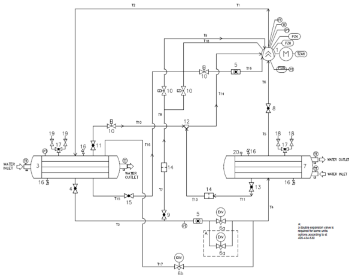
Figur 14 - P&ID Option 251
