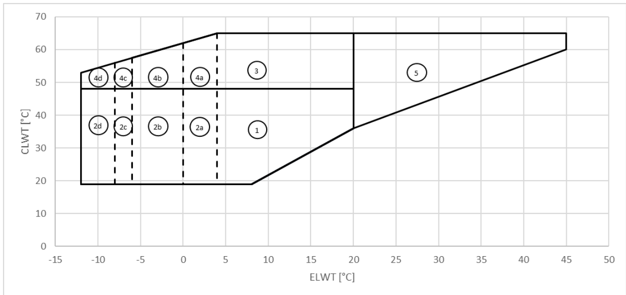
Figura6 - EWWD-VZ-XS/PS
