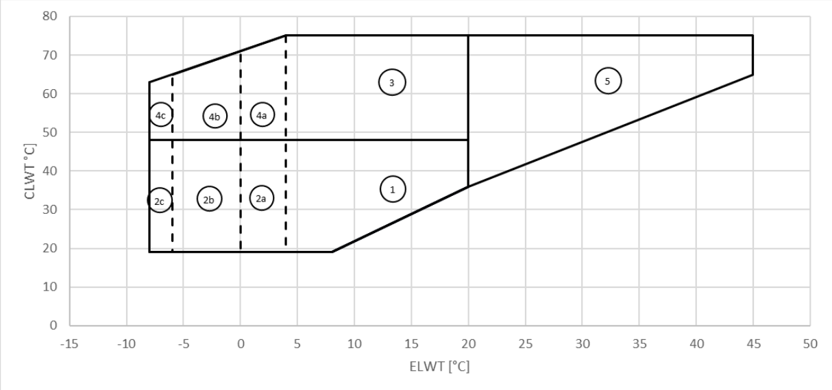
Figura8 - EWWH_VZ_XS
