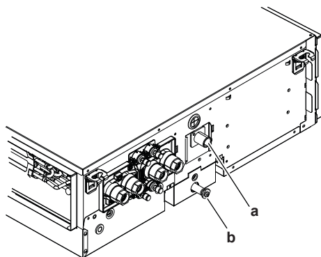
a Dreneringsmuffe b Gummiplugg
