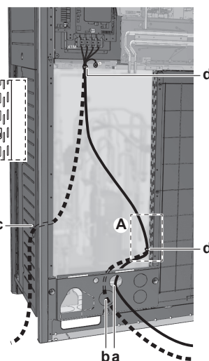
14~20 HP
