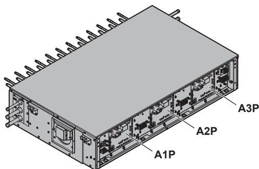
A1P PCB principal A1P
