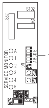
1 Innstillingsbryter for prioritert rom SW4
