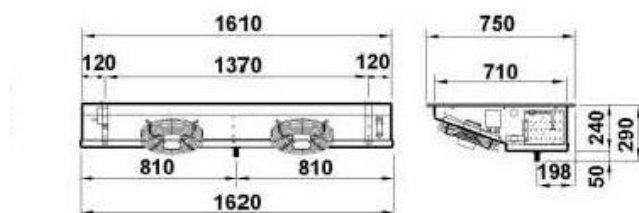
Evaporator GS340
