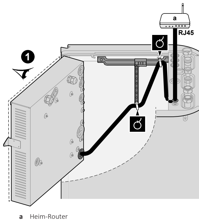
a Heim-Router
