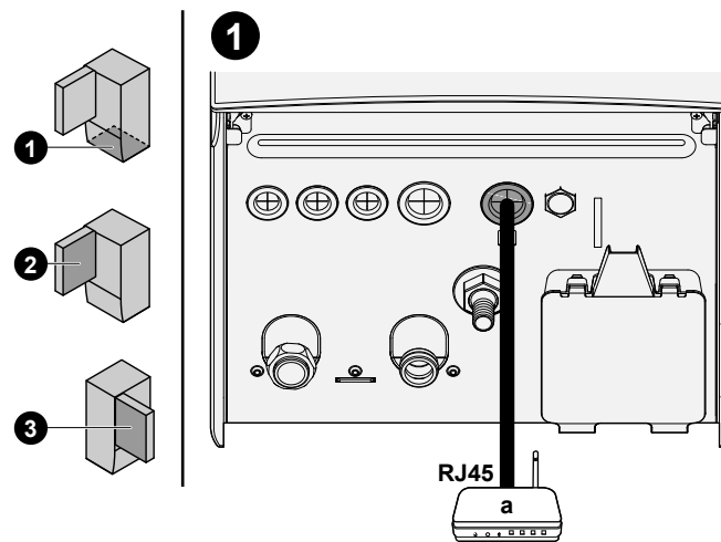
a Heim-Router
