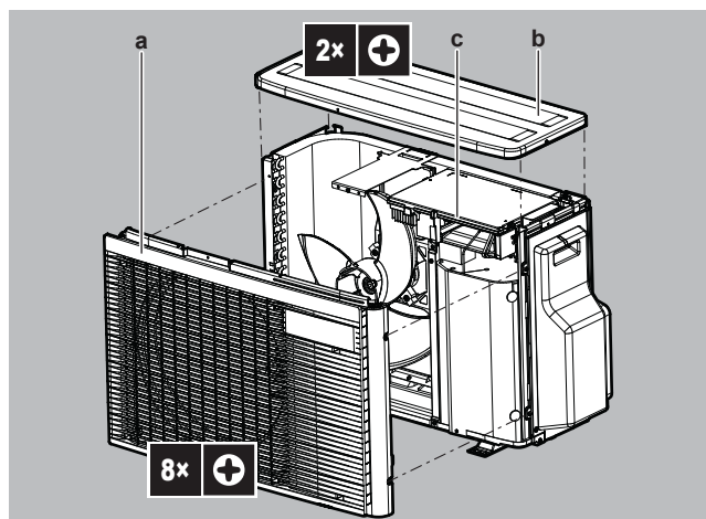
a Frontplate
